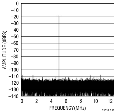
LTC2203: 32K Point FFT, f_{IN} = 30\text{MHz} , -20dBFS, PGA = 1
