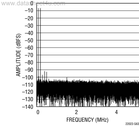
LTC2202: 32K Point 2-Tone FFT, f_{IN} = 60.2\text{MHz} and 70.1\text{MHz} , -7\text{dBFS} , \text{PGA} = 0
